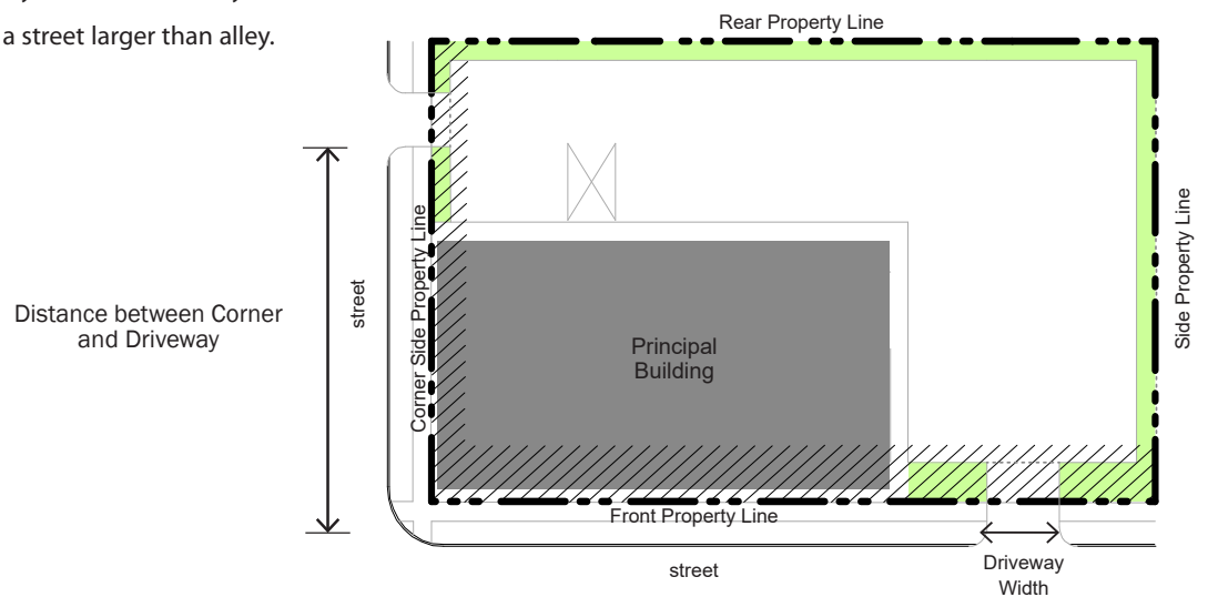
Figure 9.5 (1). Driveway Width and Location.
