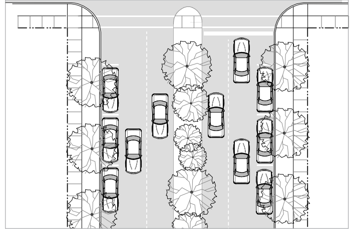
Figure 4.3 (3). Wide Street Crossing with Pedestrian Refuge Median.
